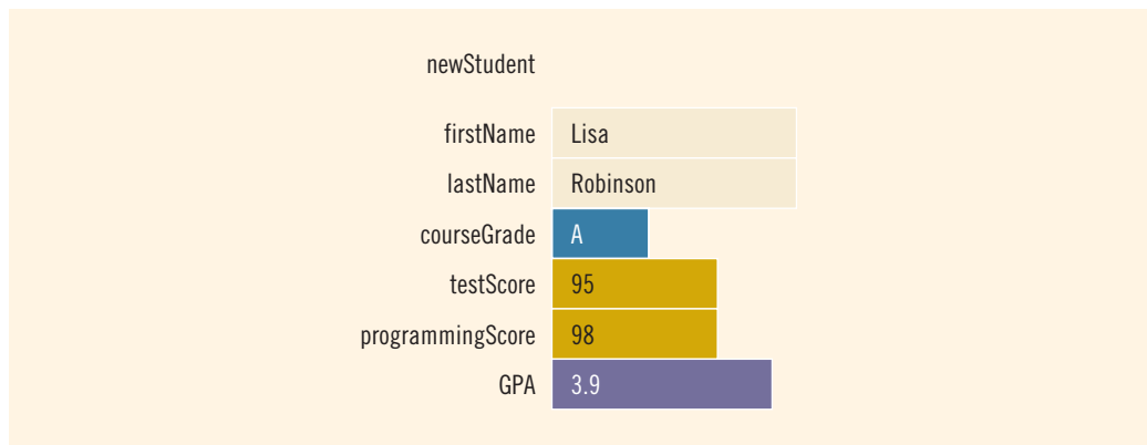
FIGURE 11-3 struct newStudent
