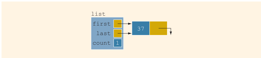
FIGURE 18-22 list with one node
