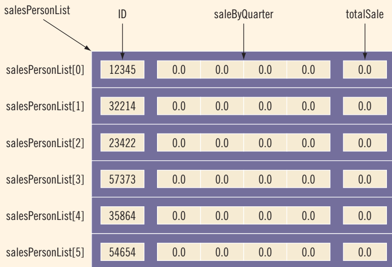
FIGURE 11-10 Array salesPersonList after initialization
