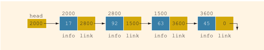
FIGURE 18-4 Linked list with four nodes
