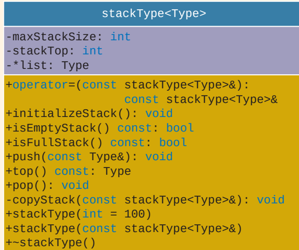
FIGURE 19-5 UML class diagram of the class stackType
