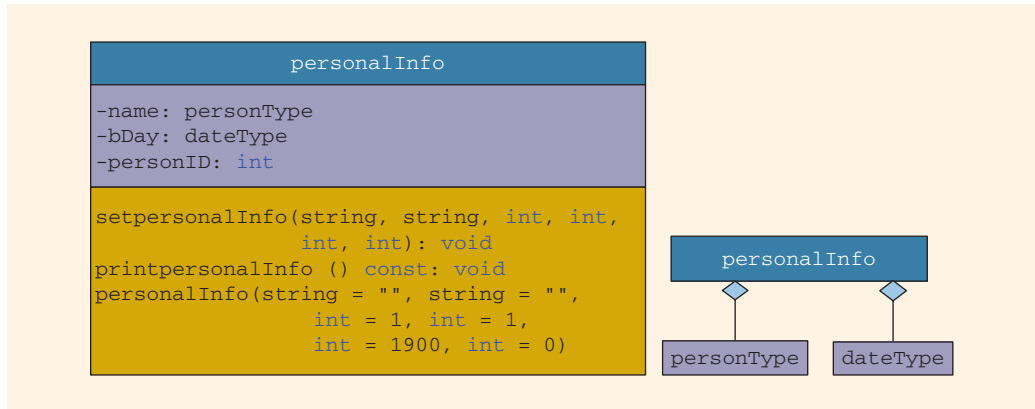
FIGURE 13-8 UML class diagram of the class personalInfo and composition (aggregation)
