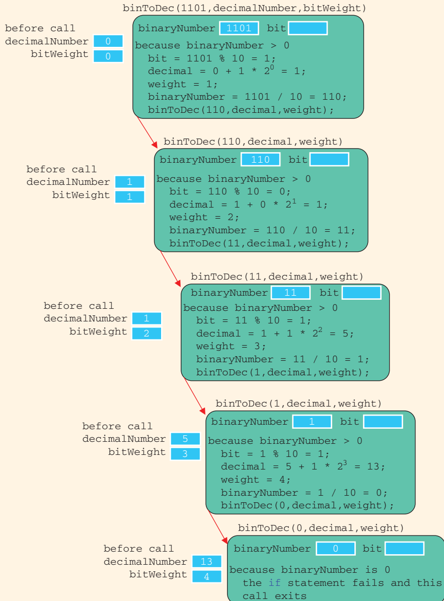
FIGURE 17-8 Execution of binToDec(1101, decimalNumber, bitWeight);
