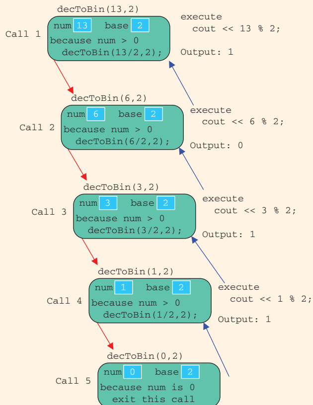
FIGURE 17-9 Execution of decToBin(13, 2)
