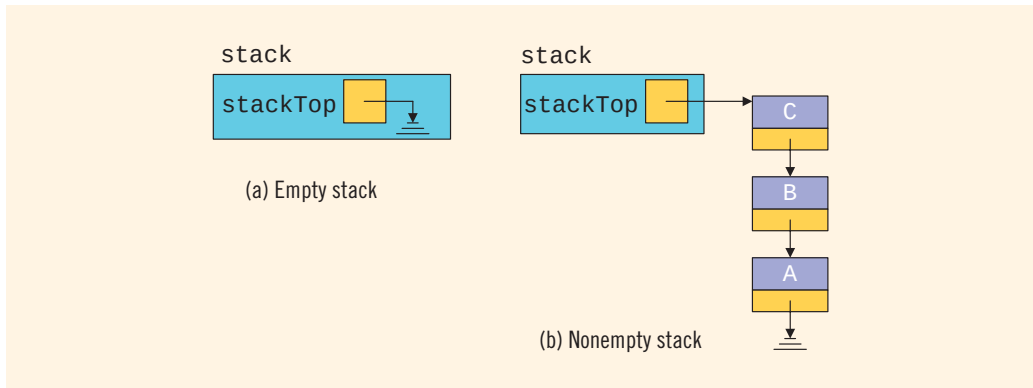
FIGURE 19-12 Empty and nonempty linked stack
