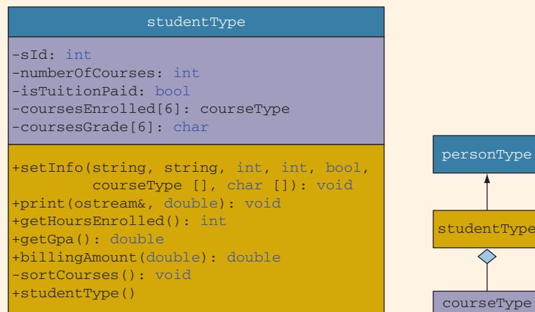
FIGURE 13-10 UML class diagram of the class studentType together with inheritance and composition (aggregation) relation
