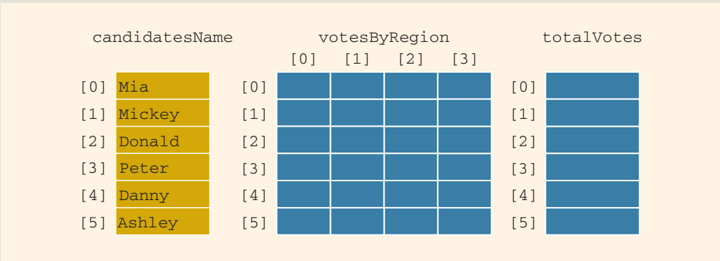
FIGURE 10-21 Arrays candidatesName , votesByRegion , and totalVotes after reading candidates' names
