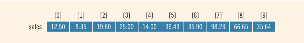
FIGURE 9-6 Array sales
