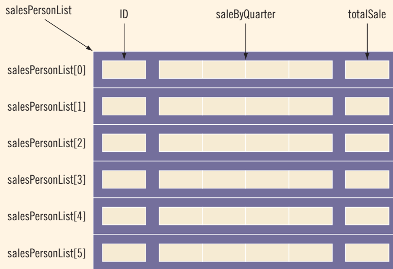
FIGURE 11-9 Array salesPersonList
