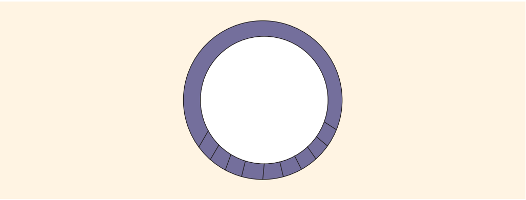
FIGURE 19-30 Circular queue
